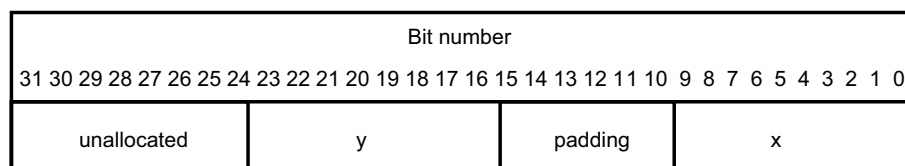
Figure 6-2 Bitfield allocation 1
